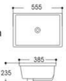
LX-6217 Under Counter Basin Outside Size:555x385x235mm 21 7/8"x15 1/4"x9 1/4" Inside Size:495x325mm 19 1/2"x12 3/4" Under counter mounting
