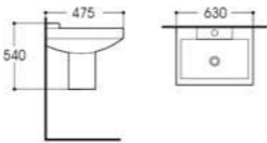
LX-3732H Wall-hung Basin Size:630x475x540mm Vitreous china Fixing to wall with back
