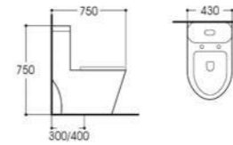
LX-2001 Siphonic One-piece Toilet Size:750x430x750mm Vitreous china S-trap,300/400 Rounghing-in
