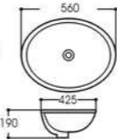
LX-6234 Under Counter Basin Outside Size:560x425x190mm 22"x16 3/4"x7 1/2" Inside Size:510x370mm 20 1/8"x14 5/8" Under counter mounting
