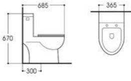
LX-2734 Siphonic One-piece Toilet Size:685x365x670mm Vitreous china S-trap,300mm Rounghing-in
