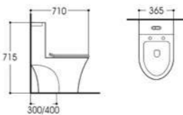
LX-2054 Rimless Siphonic One-piece Toilet Size:710x365x715mm Vitreous china S-trap,300/400mm Rounghing-in
