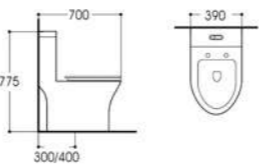
LX-2701 Rimless Siphonic One-piece Toilet Size:700x390x775mm Vitreous china S-trap,300/400mm Rounghing-in
