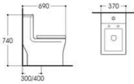
LX-2093 Siphonic One-piece Toilet Size:690x370x740mm Vitreous china S-trap,300/400mm Rounghing-in
