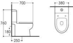
LX-2755 Wasdown Two-piece Toilet Size:700x380x760mm Vitreous china S-trap,250mm Rounghing-in P-trap,180mmRounghing-in
