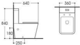
LX-2905 Washdown Two-piece Toilet Size:640x360x840mm Vitreous china S-trap,250mm Rounghing-in P-trap,180mm Rounghing-in
