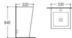
LX-8014 Pedestal Basin Size:330x320x840mm Vitreous china Fixing to wall with back
