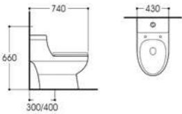
LX-2122 Rimless Siphonic One-piece Toilet Size:740x430x660mm Vitreous china S-trap,300/400mm Rounghing-in
