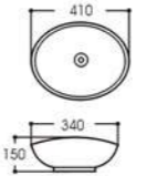
LX-7122 Art basin Size:410x340x150mm Vitreous china Above counter mounting
