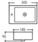
LX-5402 Hanging basin Size:300x185x95mm Vitreous china Hanging installation
