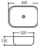
LX-7114 Art basin Size:455x325x135mm Vitreous china Above counter mounting
