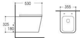
LX-1907 Washdown Wall-hung Toilet Size:530x355x325mm Vitreous china P-trap,180mm Rounghing-in
