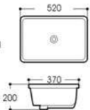
LX-6108 Under Counter Basin Outside Size:520x370x200mm 20 1/2"x14 5/8"x7 7/8" Inside Size:465x320mm 18 1/4"x12 5/8" Under counter mounting
