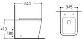
LX-1908 Floor standing toilet Size:540x345x410mm Vitreous china P-trap,180mm Rounghing-in
