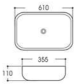
LX-7043 Art basin Size:610x355x110mm Vitreous china Above counter mounting
