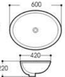
LX-6237 Under Counter Basin Outside Size:600x420x220mm 23 5/8"x16 1/2"x8 3/4" Inside Size:550x370mm 21 3/4"x14 5/8" Under counter mounting
