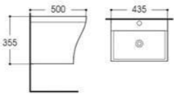
LX-3001 Wall-hung basin Size:435x500x355mm Vitreous china Fixing to wall with back
