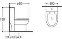
LX-2083 Siphonic/Washdown One-piece Toilet Size:680x380x730mm Vitreous china S-trap,200/300/400mm Rounghing-in
