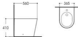
LX-1057A Floor Standing Bidet Size:560x365x410mm Vitreous china Fixing to wall with back
