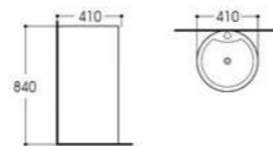
LX-8019 Pedestal Basin Size:410x410x840mm Vitreous china Fixing to wall with back
