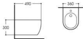
LX-1006 Bidet Size:490x360x300mm Vitreous china Fixing to wall with back
