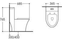
LX-2722 Rimless Siphonic One-piece Toilet Size:685x365x765mm Vitreous china S-trap,300/400mm Rounghing-in
