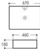
LX-5187 Art basin Size:670x460x150mm Vitreous china Above counter mounting
