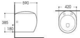
LX-1038 Washdown Wall-hung Toilet Size:590x420x385mm Vitreous china P-trap,180mm Rounghing-in
