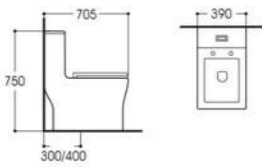
LX-2038 Rimless Siphonic One-piece Toilet Size:705x390x750mm Vitreous china S-trap,300/400mm Rounghing-in
