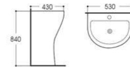
LX-8011 Pedestal Basin Size:530x430x840mm Vitreous china Fixing to wall with back
