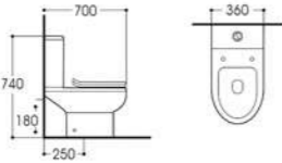
LX-2758 Wasdown Two-piece Toilet Size:700x360x740mm Vitreous china S-trap,250mm Rounghing-in P-trap,180mmRounghing-in
