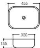
LX-C020 Art basin Size:455x320x135mm Vitreous china Above counter mounting
