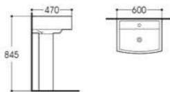
LX-3003F Pedestal Basin Size: 600x470x845mm Vitreous china Fixing to wall with back
