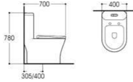
LX-2129 Rimless Siphonic One-piece Toilet Size:700x400x780mm Vitreous china S-trap,305/400 Rounghing-in
