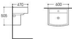
LX-3003H Wall-hung Basin Size:600X470X505mm Vitreous china Fixing to wall with back
