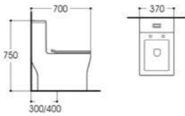
LX-2079 Rimless Siphonic One-piece Toilet Size:700x370x750mm Vitreous china S-trap,300/400 Rounghing-in
