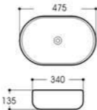
LX-5608 Art basin Size:475x340x135mm Vitreous china Above counter mounting
