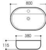
LX-5590 Art basin Size:800x380x115mm Vitreous china Above counter mounting
