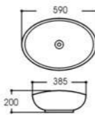
LX-5150 Art basin Size:590x385x200mm Vitreous china Above counter mounting
