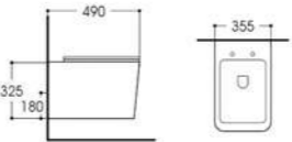
LX-1148 Rimless Washdown Wall-hung Toilet Size:490x355x325mm Vitreous china P-trap,180mm Rounghing-in
