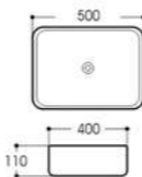
LX-7042 Art basin Size:500x400x110mm Vitreous china Above counter mounting
