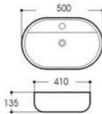
LX-5592 Art basin Size:500x410x135mm Vitreous china Above counter mounting
