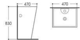
LX-8006 Pedestal Basin Size:470x470x830mm Vitreous china Fixing to wall with back
