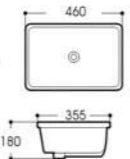
LX-6207 Under Counter Basin Outside Size:460x355x180mm 18 1/8"x14"x7" Inside Size:410x305mm 16 1/8"x12" Under counter mounting
