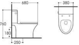
LX-2760 Wasdown Two-piece Toilet Size:680x380x760mm Vitreous china S-trap,250mm Rounghing-in P-trap,180mmRounghing-in
