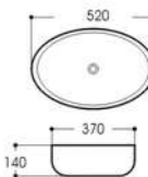
LX-5605 Art basin Size:520x370x140mm Vitreous china Above counter mounting
