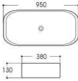
LX-5450 Art basin Size:950x380x130mm Vitreous china Above counter mounting
