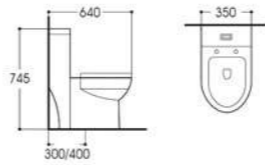
LX-2090 Rimless Siphonic One-piece Toilet Size:640x350x745mm Vitreous china S-trap,300/400mm Rounghing-in
