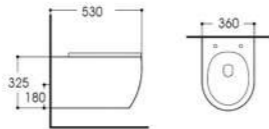
LX-1106L Rimless Washdown Wall-hung Toilet Size:530x360x325mm Vitreous china P-trap,180mm Rounghing-in
