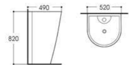
LX-8002 Pedestal Basin Size:520x490x820mm Vitreous china Fixing to wall with back
