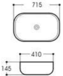
LX-5420 Art basin Size:715x410x145mm Vitreous china Above counter mounting
