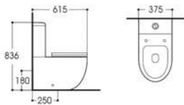
LX-2903 Washdown Two-piece Toilet Size:615x375x836mm Vitreous china S-trap,250 Rounghing-in P-trap,180mm Rounghing-in
