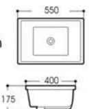
LX-6224 Under Counter Basin Outside Size:550x400x175mm 21 3/4"x15 3/4"x6" 7/8" Inside Size:000x000mm 19 3/4"x13 3/4" Under counter mounting
