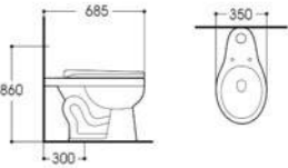
LX-1008 Wasdown Two-piece Toilet Size:685x350x860mm Vitreous china S-trap,300mm Rounghing-in
