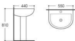
LX-3206F Pedestal Basin Size:550x440x810mm Vitreous china Fixing to wall with back
