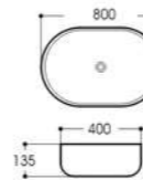
LX-5600 Art basin Size:800x400x135mm Vitreous china Above counter mounting
