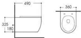
LX-1106 Rimless Washdown Wall-hung Toilet Size:490x360x325mm Vitreous china P-trap,180mm Rounghing-in
