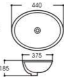
LX-6224 Under Counter Basin Outside Size:440x375x185mm 17 3/8"x14 3/4"x7 1/4" Inside Size:400x335mm 15 3/4"x13 1/5" Under counter mounting
