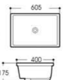
LX-6222 Under Counter Basin Outside Size:605x400x175mm 23 3/4"x15 3/4"x7" 1/8" Inside Size:545x340mm 21 1/2"x13 3/8" Under counter mounting
