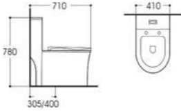
LX-2130 Rimless Siphonic One-piece Toilet Size:710x410x780mm Vitreous china S-trap,305/400 Rounghing-in
