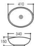
LX-7128 Art basin Size:410x340x150mm Vitreous china Above counter mounting
