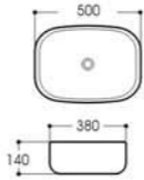
LX-5502 Art basin Size:500x380x140mm Vitreous china Above counter mounting
