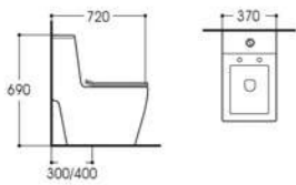
LX-2906 Rimless Siphonic One-piece Toilet Size:720x370x690mm Vitreous china S-trap,300/400 Rounghing-in
