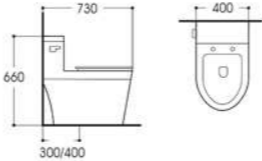
LX-2535B Rimless Siphonic One-piece Toilet Size:730x400x660mm Vitreous china S-trap,300/400mm Rounghing-in
