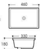
LX-6202 Under Counter Basin Outside Size:460x330x180mm 18 1/8"x13x7" 1/8" Inside Size:410x278mm 16 1/8"x11" Under counter mounting
