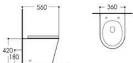
LX-1906 Floor standing toilet Size:560x360x420mm Vitreous china P-trap,180mm Rounghing-in
