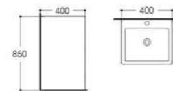
LX-8009 Pedestal Basin Size:400x400x850mm Vitreous china Fixing to wall with back
