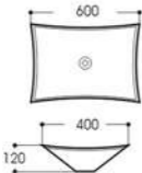
LX-5330 Art basin Size:600x400x120mm Vitreous china Above counter mounting
