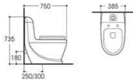
LX-2080 Washdown One-piece Toilet Size:750x385x735mm Vitreous china S-trap,250/300mm Rounghing-in P-trap,180mm Rounghing-in
