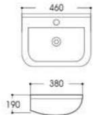
LX-5620 Wall-hung Basin Size:460x380x190mm Vitreous china Fixing to wall with back
