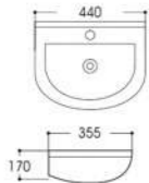
LX-5619 Wall-hung Basin Size:440x355x170mm Vitreous china Fixing to wall with back
