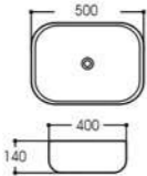
LX-C011 Art basin Size:500x400x140mm Vitreous china Above counter mounting
