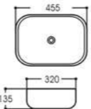
LX-C021 Art basin Size:455x320x135mm Vitreous china Above counter mounting
