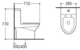
LX-2888 Siphonic One-piece Toilet Size:710x385x770mm Vitreous china S-trap,300/400 Rounghing-in
