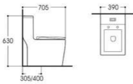
LX-2039 Rimless Siphonic One-piece Toilet Size:705x390x630mm Vitreous china S-trap,305/400mm Rounghing-in
