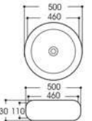
LX-5263A/5263B Art basin Size A:500x500x130mm Size B:460x460x110mm Above counter mounting
