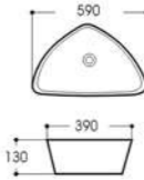
LX-5565 Art basin Size:590x390x130mm Vitreous china Above counter mounting
