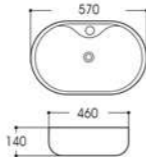
LX-5457 Art basin Size:570x460x140mm Vitreous china Above counter mounting
