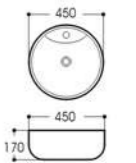
LX-5602 Art basin Size:450x450x170mm Vitreous china Above counter mounting
