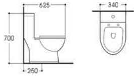
LX-2068 Siphonic One-piece Toilet Size:625x340x700mm Vitreous china S-trap,250mm Rounghing-in
