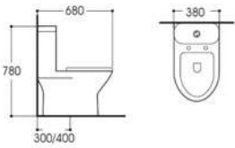
LX-2920 Siphonic One-piece Toilet Size:680x380x780mm Vitreous china S-trap,300/400 Rounghing-in
