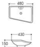
LX-5517 Art basin Size:480x430x150mm Vitreous china Above counter mounting
