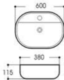
LX-5589 Art basin Size:600x380x115mm Vitreous china Above counter mounting
