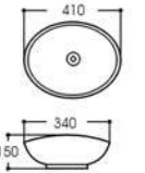
LX-7123 Art basin Size:410x340x150mm Vitreous china Above counter mounting
