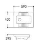
LX-4151 Squatting Pan W.C Size:590x460x295mm Vitreous china Fixing to wall with back
