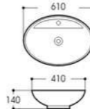
LX-5802 Art basin Size: 610x410x140mm Vitreous china Above counter mounting
