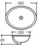
LX-6245 Under Counter Basin Outside Size:360x300x165mm 14 1/4"x11 4/5"x6 1/2" Inside Size:320x265mm 12 3/5"x10 2/5" Under counter mounting
