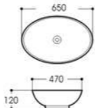
LX-5346 Art basin Size:650x470x120mm Vitreous china Above counter mounting
