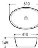
LX-5601 Art basin Size:610x410x145mm Vitreous china Above counter mounting
