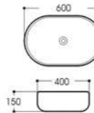
LX-C113 Art basin Size:600x400x150mm Vitreous china Above counter mounting
