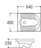
LX-3804 Squatting Pan W.C Size:540x450x230mm Vitreous china Fixing to wall with back
