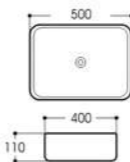
LX-7041 Art basin Size:500x400x110mm Vitreous china Above counter mounting
