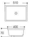
LX-6218 Under Counter Basin Outside Size:510x400x170mm 20 1/8"x15 3/4"x6 3/4" Inside Size:440x330mm 17 1/4"x13 Under counter mounting
