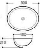
LX-6236 Under Counter Basin Outside Size:530x400x210mm 20 7/8"x15 3/4"x8 1/4" Inside Size:480x350mm 18 7/8"x13 3/4" Under counter mounting
