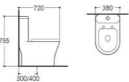
LX-2094 Rimless Siphonic One-piece Toilet Size:720x380x755mm Vitreous china S-trap,300/400mm Rounghing-in
