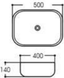
LX-C009 Art basin Size:500x400x140mm Vitreous china Above counter mounting
