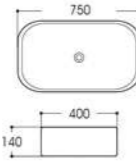
LX-5419 Art basin Size:750x400x140mm Vitreous china Above counter mounting
