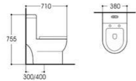
LX-2091 Siphonic One-piece Toilet Size:710x380x755mm Vitreous china S-trap,300/400 Rounghing-in
