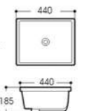
LX-6223 Under Counter Basin Outside Size:440x440x185mm 17 3/8"x17 3/8"x7" 1/4" Inside Size:380x380mm 15"x15" Under counter mounting
