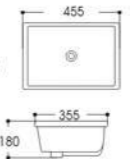
LX-6220 Under Counter Basin Outside Size:455x355x180mm 18"x14"x7 1/8" Inside Size:395x295mm 15 5/8"x11 1/2" Under counter mounting
