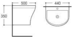
LX-3006 Wall-hung basin Size:440x500x350mm Vitreous china Fixing to wall with back
