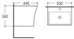
LX-3004 Wall-hung basin Size:530x440x360mm Vitreous china Fixing to wall with back
