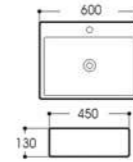
LX-5804B Art basin Size:600x450x130mm Vitreous china Above counter mounting
