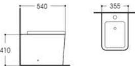
LX-1062 Floor standing Bidet Size:540x355x410mm Vitreous china Fixing to wall with back
