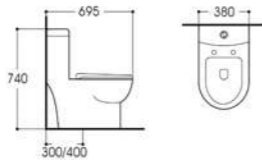
LX-2064 Rimless Siphonic One-piece Toilet Size:695x380x740mm Vitreous china S-trap,300/400 Rounghing-in
