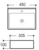
LX-5277 Art basin Size:450x305x100mm Vitreous china Above counter mounting
