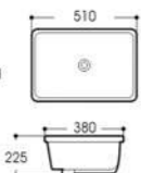
LX-6210 Under Counter Basin Outside Size:510x380x225mm 20"x15x8" 7/8" Inside Size:460x330mm 18 1/8"x13" Under counter mounting
