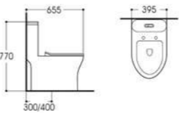
LX-2179 Siphonic One-piece Toilet Size:655x395x770mm Vitreous china S-trap,300/400mm Rounghing-in
