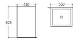
LX-8010 Pedestal Basin Size:530x430x825mm Vitreous china Fixing to wall with back
