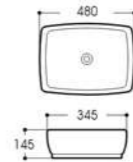
LX-5240A Art basin Size:480x345x145mm Vitreous china Above counter mounting
