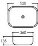
LX-5544 Art basin Size:520x360x135mm Vitreous china Above counter mounting
