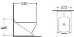
LX-1190 Bidet Size:530x370x445mm Vitreous china Fixing to wall with back
