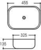
LX-7115 Art basin Size:455x325x135mm Vitreous china Above counter mounting
