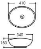
LX-7124 Art basin Size:410x340x150mm Vitreous china Above counter mounting
