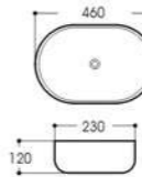
LX-5415 Art basin Size:460x230x120mm Vitreous china Above counter mounting
