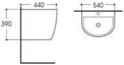
LX-3009 Wall-hung Basin Size:540x440x390mm Vitreous china Fixing to wall with back
