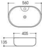
LX-5579 Art basin Size:560x405x135mm Vitreous china Above counter mounting
