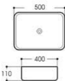
LX-7040 Art basin Size:500x400x110mm Vitreous china Above counter mounting
