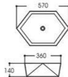
LX-5615 Art basin Size:570x360x140mm Vitreous china Above counter mounting
