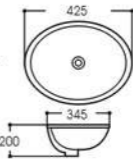
LX-6227 Under Counter Basin Outside Size:425x345x200mm 16 3/4"x13 3/5"x7 7/8" Inside Size:380x310mm 15"x12 1/4" Under counter mounting
