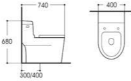
LX-2602 Rimless Siphonic One-piece Toilet Size:740x400x680mm Vitreous china S-trap,300/400mm Rounghing-in
