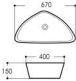
LX-5566 Art basin Size:670x400x150mm Vitreous china Above counter mounting
