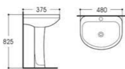
LX-3209F Pedestal Basin Size:480x375x825mm Vitreous china Fixing to wall with back
