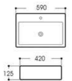
LX-5268 Art basin Size:590x420x125mm Vitreous china Above counter mounting
