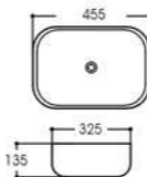
LX-7120 Art basin Size:455x325x135mm Vitreous china Above counter mounting
