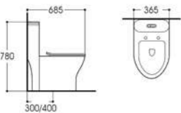
LX-2606 Rimless Siphonic One-piece Toilet Size:685x365x780mm Vitreous china S-trap,300/400mm Rounghing-in
