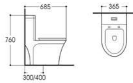
LX-2188 Rimless Siphonic One-piece Toilet Size:685x365x760mm Vitreous china S-trap,300/400mm Rounghing-in
