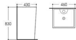
LX-8012 Pedestal Basin Size:460x430x830mm Vitreous china Fixing to wall with back
