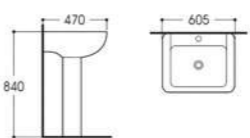
LX-3229F Pedestal Basin Size:605x470x840mm Vitreous china Fixing to wall with back
