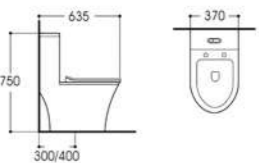
LX-2140 Rimless Siphonic One-piece Toilet Size:635x370x750mm Vitreous china S-trap,300/400mm Rounghing-in
