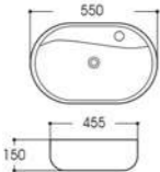
LX-5456 Art basin Size:550x455x150mm Vitreous china Above counter mounting
