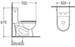
LX-2733 Siphonic One-piece Toilet Size:700x365x675mm Vitreous china S-trap,300/400mm Rounghing-in
