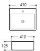
LX-5458 Art basin Size:410x410x125mm Vitreous china Above counter mounting
