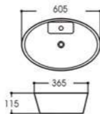
LX-5562 Art basin Size:605x365x115mm Vitreous china Above counter mounting
