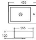
LX-5349left Hanging basin Size:455x255x120mm Vitreous china Hanging installation
