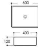
LX-5511 Art basin Size:600x400x120mm Vitreous china Above counter mounting
