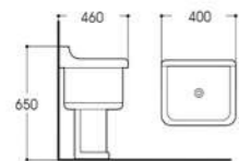
LX-3023 Mop tub Size:460x400x650mm Vitreous china Fixing to wall with back
