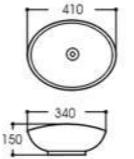
LX-7121 Art basin Size:410x340x150mm Vitreous china Above counter mounting
