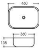
LX-5543 Art basin Size:460x360x135mm Vitreous china Above counter mounting
