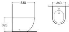
LX-1831 Floor Standing Toilet Size:530x360x325mm Vitreous china Fixing to wall with back
