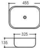
LX-7113 Art basin Size:455x325x135mm Vitreous china Above counter mounting
