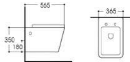
LX-1133 Washdown Wall-hung Toilet Size:565x365x350mm Vitreous china P-trap,180mm Rounghing-in
