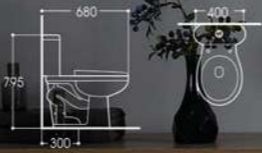
LX-2759A Siphonic Two-piece Toilet Size:680x400x795mm Vitreous china S-trap,300mm Rounghing-in
