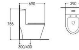
LX-2111 Rimless Siphonic One-piece Toilet Size:690x390x755mm Vitreous china S-trap,300/400 Rounghing-in
