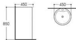
LX-8003 Pedestal Basin Size:450x450x850mm Vitreous china Fixing to wall with back
