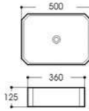
LX-5508 Art basin Size:500x360x125mm Vitreous china Above counter mounting
