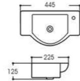
LX-5316 Hanging basin Size:445x225x125mm Vitreous china Hanging installation
