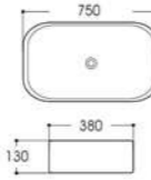
LX-5449 Art basin Size:750x380x130mm Vitreous china Above counter mounting
