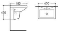
LX-3135H Wall-hung Basin Size:650x480x490mm Vitreous china Fixing to wall with back
