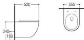
LX-1901 Rimless Washdown Wall-hung Toilet Size:520x355x340mm Vitreous china P-trap,180mm Rounghing-in
