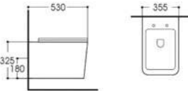
LX-1907 Washdown Wall-hung Toilet Size:530x355x325mm Vitreous china P-trap,180mm Rounghing-in
