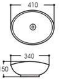
LX-7126 Art basin Size:410x340x150mm Vitreous china Above counter mounting
