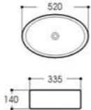
LX-5416 Art basin Size:520x335x140mm Vitreous china Above counter mounting
