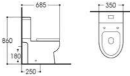
LX-2599ADA Wasdown Two-piece Toilet Size:685x350x860mm Vitreous china S-trap,250mm Rounghing-in P-trap,180mmRounghing-in
