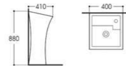
LX-8015 Pedestal Basin Size:400x410x880mm Vitreous china Fixing to wall with back
