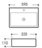
LX-5278 Art basin Size:595x325x110mm Vitreous china Above counter mounting
