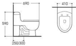
LX-2109 Siphonic One-piece Toilet Size:690x410x590mm Vitreous china S-trap,250/300mm Rounghing-in
