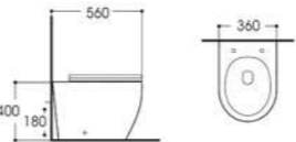
LX-1902 Floor standing toilet Size:560x360x400mm Vitreous china P-trap,180mm Rounghing-in
