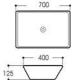
LX-5272 Art basin Size:700x400x125mm Vitreous china Above counter mounting
