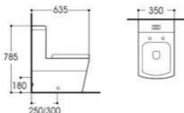
LX-2003 Washdown One-piece Toilet Size:635x350x785mm Vitreous china S-trap,250/300mm Rounghing-in P-trap,180mm Rounghing-in
