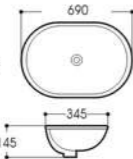
LX-6243 Under Counter Basin Outside Size:690x345x145mm 27 1/8"x13 1/2"x5 3/4" Inside Size:640x295mm 25 1/4"x11 5/8" Under counter mounting
