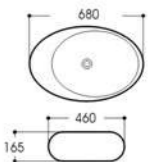
LX-5572 Art basin Size:680x460x165mm Vitreous china Above counter mounting
