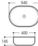
LX-5302 Art basin Size:540x400x145mm Vitreous china Above counter mounting
