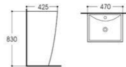
LX-8008 Pedestal Basin Size:470x425x830mm Vitreous china Fixing to wall with back
