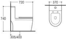
LX-2112 Rimless Siphonic One-piece Toilet Size:720x370x740mm Vitreous china S-trap,305/400 Rounghing-in
