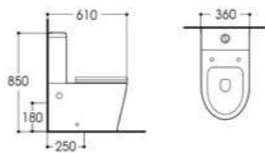
LX-2904 Washdown Two-piece Toilet Size:610x360x850mm Vitreous china S-trap,250 Rounghing-in P-trap,180mm Rounghing-in
