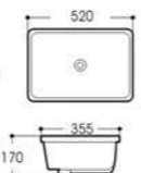
LX-6211 Under Counter Basin Outside Size:520x355x170mm 20 1/2"x14x6" 1/2" Inside Size:470x300mm 18 1/2"x12" Under counter mounting
