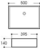
LX-5507 Art basin Size:500x395x140mm Vitreous china Above counter mounting
