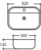
LX-5542 Art basin Size:520x360x140mm Vitreous china Above counter mounting
