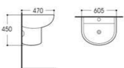
LX-3229H Wall-hung Basin Size:605x470x450mm Vitreous china Fixing to wall with back
