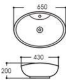
LX-5043 Art basin Size:650x430x200mm Vitreous china Above counter mounting
