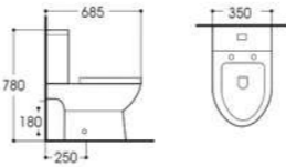
LX-2599 Wasdown Two-piece Toilet Size:685x350x780mm Vitreous china S-trap,250mm Rounghing-in P-trap,180mmRounghing-in
