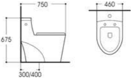
LX-2913 Siphonic One-piece Toilet Size:750x460x675mm Vitreous china S-trap,300/400mm Rounghing-in
