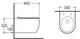
LX-1106 Rimless Washdown Wall-hung Toilet Size:490x360x325mm Vitreous china P-trap,180mm Rounghing-in
