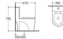
LX-2092 Rimless Siphonic One-piece Toilet Size:670x390x790mm Vitreous china S-trap,250/300/400 Rounghing-in
