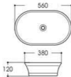
LX-5412 Art basin Size:560x380x120mm Vitreous china Above counter mounting
