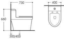
LX-2535A Rimless Siphonic One-piece Toilet Size:730x400x660mm Vitreous china S-trap,300/400mm Rounghing-in
