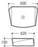
LX-5222 Art basin Size:600x425x150mm Vitreous china Above counter mounting
