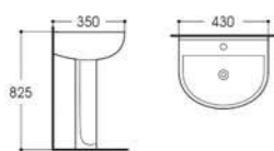
LX-3210F Pedestal Basin Size:430x350x825mm Vitreous china Fixing to wall with back
