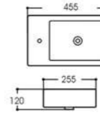
LX-5349right Hanging basin Size:455x255x120mm Vitreous china Hanging installation
