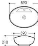
LX-5001 Art basin Size:590x390x210mm Vitreous china Above counter mounting
