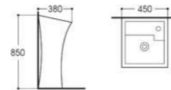
LX-8013 Pedestal Basin Size:450x380x850mm Vitreous china Fixing to wall with back
