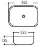
LX-7116 Art basin Size:455x325x135mm Vitreous china Above counter mounting
