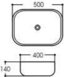
LX-C007 Art basin Size:500x400x140mm Vitreous china Above counter mounting
