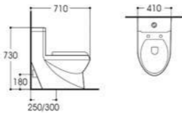
LX-2081 Washdown One-piece Toilet Size:710x410x730mm Vitreous china S-trap,250/300mm Rounghing-in P-trap,180mm Rounghing-in
