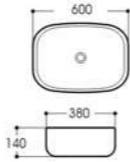
LX-5503 Art basin Size:600x380x140mm Vitreous china Above counter mounting
