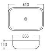
LX-7045 Art basin Size:610x355x110mm Vitreous china Above counter mounting
