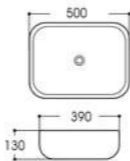
LX-7039 Art basin Size:500x390x130mm Vitreous china Above counter mounting
