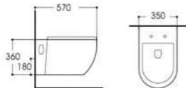
LX-1115 Rimless Washdown Wall-hung Toilet Size:570x350x360mm Vitreous china P-trap,180mm Rounghing-in
