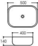
LX-C008 Art basin Size:500x400x140mm Vitreous china Above counter mounting
