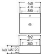
LX-5079A 5079B/5079C Art basin Size:A460X460X160mm Size:B410X410X145mm Size:C380X380X120mm
