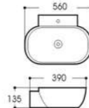
LX-5390 Art basin Size:560x390x135mm Vitreous china Above counter mounting
