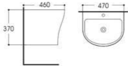
LX-3007 Wall-hung basin Size:470x460x370mm Vitreous china Fixing to wall with back
