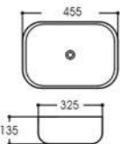
LX-7118 Art basin Size:455x325x135mm Vitreous china Above counter mounting
