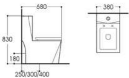
LX-2135 Siphonic/Washdown One-piece Toilet Size:680x380x830mm Vitreous china S-trap,250/300/400mm Rounghing-in P-trap,180mm Rounghing-in
