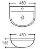
LX-5376 Hanging basin Size:430x430x185mm Vitreous china Hanging installation
