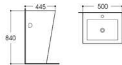
LX-8005 Pedestal Basin Size:500x445x840mm Vitreous china Fixing to wall with back
