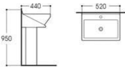
LX-3190 Pedestal Basin Size:520x440x950mm Vitreous china Fixing to wall with back
