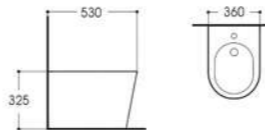
LX-1057 Bidet Size:530x360x325mm Vitreous china Fixing to wall with back
