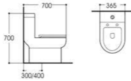
LX-2007 Siphonic One-piece Toilet Size:700x365x700mm Vitreous china S-trap,300/400 Rounghing-in
