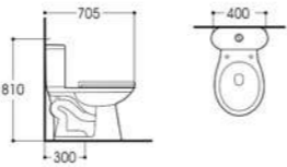
LX-2756A Siphonic Two-piece Toilet Size:705x400x810mm Vitreous china S-trap,300mm Rounghing-in
