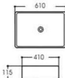
LX-5253 Art basin Size:610x410x115mm Vitreous china Above counter mounting
