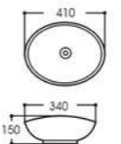
LX-7127 Art basin Size:410x340x150mm Vitreous china Above counter mounting
