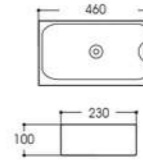
LX-5375 Hanging basin Size:460x230x100mm Vitreous china Hanging installation
