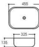
LX-7119 Art basin Size:455x325x135mm Vitreous china Above counter mounting
