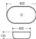
LX-5594 Art basin Size:800x400x135mm Vitreous china Above counter mounting
