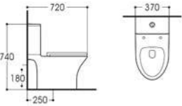
LX-2777 Wasdown Two-piece Toilet Size:720x370x740mm Vitreous china S-trap,250mm Rounghing-in P-trap,180mmRounghing-in
