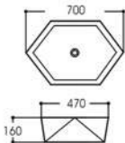
LX-5617 Art basin Size:700x470x160mm Vitreous china Above counter mounting
