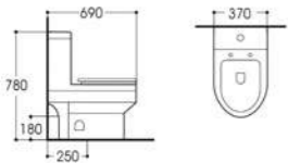
LX-2732 Washdown One-piece Toilet Size:690x370x780mm Vitreous china S-trap,250mm Rounghing-in P-trap,180mm Rounghing-in
