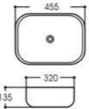
LX-C018 Art basin Size:455x320x135mm Vitreous china Above counter mounting
