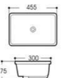
LX-6212 Under Counter Basin Outside Size:455x300x175mm 17 7/8"x11 3/4"x6" 7/8" Inside Size:415x250mm 16 1/4"x9 3/4" Under counter mounting
