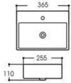
LX-5338 Hanging basin Size:365x255x110mm Vitreous china Hanging installation
