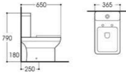
LX-2830 Wasdown Two-piece Toilet Size:650x365x790mm Vitreous china S-trap,250mm Rounghing-in P-trap,180mmRounghing-in
