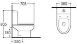
LX-2023 Wasdown Two-piece Toilet Size:705x380x805mm Vitreous china S-trap,250mm Rounghing-in P-trap,180mmRounghing-in
