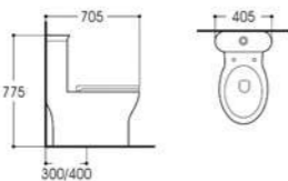
LX-2041 Rimless Siphonic One-piece Toilet Size:705x405x775mm Vitreous china S-trap,300/400mm Rounghing-in
