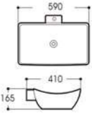
LX-5391 Art basin Size:590x410x165mm Vitreous china Above counter mounting
