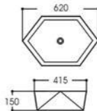
LX-5616 Art basin Size:620x415x150mm Vitreous china Above counter mounting
