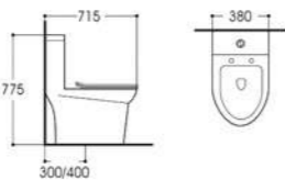
LX-2704 Rimless Siphonic One-piece Toilet Size:715x380x775mm Vitreous china S-trap,300/400mm Rounghing-in
