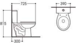
LX-2749A Siphonic Two-piece Toilet Size:725x390x815mm Vitreous china S-trap,300mm Rounghing-in
