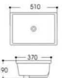
LX-6215 Under Counter Basin Outside Size:510x370x190mm 20"x14 5/8"x97" 1/2" Inside Size:460x320mm 18 1/8"x12 5/8" Under counter mounting
