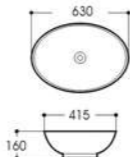
LX-5195 Art basin Size:630x415x160mm Vitreous china Above counter mounting
