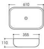
LX-7044 Art basin Size:610x355x110mm Vitreous china Above counter mounting
