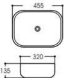
LX-C019 Art basin Size:455x320x135mm Vitreous china Above counter mounting
