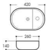
LX-5596 Art basin Size:420x260x140mm Vitreous china Above counter mounting
