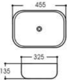
LX-7112 Art basin Size:455x325x135mm Vitreous china Above counter mounting
