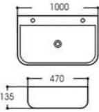
LX-5539 Art basin Size:1000X470X135mm Vitreous china Above counter mounting
