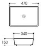
LX-5446 Art basin Size:470x340x150mm Vitreous china Above counter mounting
