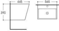
LX-3002 Wall-hung basin Size:565x445x390mm Vitreous china Fixing to wall with back
