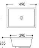
LX-6216 Under Counter Basin Outside Size:490x390x235mm 19 1/4"x15 3/8"x9" 1/4" Inside Size:420x320mm 16 1/2"x12 1/2" Under counter mounting
