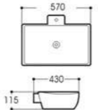
LX-5360 Art basin Size:570x430x115mm Vitreous china Above counter mounting
