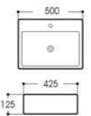
LX-5267 Art basin Size:500x425x125mm Vitreous china Above counter mounting
