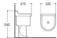
LX-3029 Mop tub Size:320x375x540mm Vitreous china Fixing to wall with back
