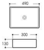
LX-5293 Art basin Size:490x300x130mm Vitreous china Above counter mounting
