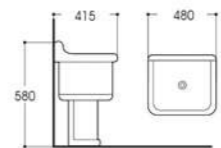
LX-3038 Mop tub Size:480x415x580mm Vitreous china Fixing to wall with back
