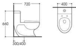
LX-2049 Washdown One-piece Toilet Size:720x400x660mm Vitreous china S-trap,300/400mm Rounghing-in
