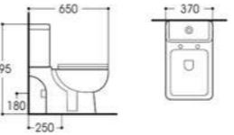
LX-2029 Wasdown Two-piece Toilet Size:650x370x795mm Vitreous china S-trap,250mm Rounghing-in P-trap,180mmRounghing-in
