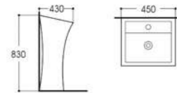
LX-8016 Pedestal Basin Size:450x430x830mm Vitreous china Fixing to wall with back
