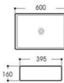
LX-5262 Art basin Size:600x395x160mm Vitreous china Above counter mounting
