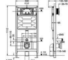
LX-3807 Concealed water tank Full/half Flush bottom Single steel Frame
