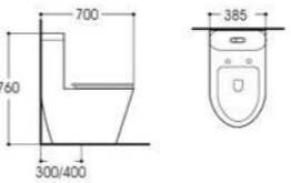
LX-2728 Rimless Siphonic One-piece Toilet Size:700x385x760mm Vitreous china S-trap,300/400 Rounghing-in
