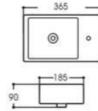
LX-5325right Hanging basin Size:365x185x90mm Vitreous china Hanging installation
