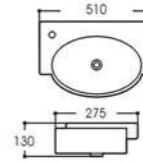
LX-5329 Hanging basin Size:510x275x130mm Vitreous china Hanging installation
