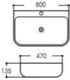
LX-5538 Art basin Size:800X470X135mm Vitreous china Above counter mounting
