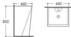
LX-8007 Pedestal Basin Size:460x460x850mm Vitreous china Fixing to wall with back
