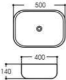
LX-C010 Art basin Size:500x400x140mm Vitreous china Above counter mounting
