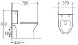
LX-2750 Wasdown Two-piece Toilet Size:720x370x750mm Vitreous china S-trap,250mm Rounghing-in P-trap,180mmRounghing-in
