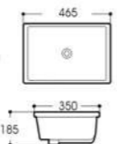
LX-6110 Under Counter Basin Outside Size:465x350x185mm 18 1/4"x13 3/4"x7" 1/4" Inside Size:415x300mm 16 1/4"x11 3/4" Under counter mounting
