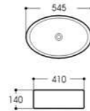
LX-5633 Art basin Size:545x410x140mm Vitreous china Above counter mounting
