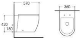
LX-1125 Washdown Close-couched Toilet Size:570x360x420mm Vitreous china P-trap,180mm Rounghing-in
