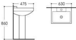
LX-3732F Pedestal Basin Size:630x475x860mm Vitreous china Fixing to wall with back
