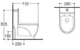
LX-2136 Washdown One-piece Toilet Size:710x380x825mm Vitreous china S-trap,250mm Rounghing-in P-trap,180mm Rounghing-in
