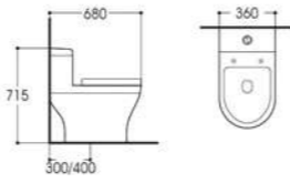
LX-2901 Siphonic One-piece Toilet Size:680x360x715mm Vitreous china S-trap,300/400mm Rounghing-in
