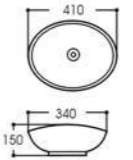
LX-7125 Art basin Size:410x340x150mm Vitreous china Above counter mounting
