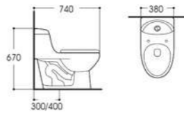
LX-2016 Siphonic One-piece Toilet Size:740x380x670mm Vitreous china S-trap,300/400mm Rounghing-in
