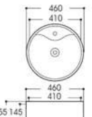
LX-5002A/5002B Art basin Size A:460x460x155mm Size B:410x410x145mm Above counter mounting
