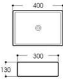
LX-5357 Art basin Size:400x300x130mm Vitreous china Above counter mounting
