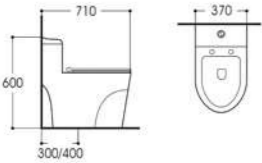
LX-2730 Siphonic One-piece Toilet Size:710x370x600mm Vitreous china S-trap,300/400mm Rounghing-in
