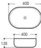
LX-5599 Art basin Size:600x400x135mm Vitreous china Above counter mounting
