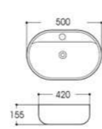
LX-5438 Art basin Size:500x420x155mm Vitreous china Above counter mounting
