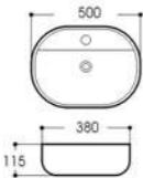
LX-5588 Art basin Size:500x380x115mm Vitreous china Above counter mounting
