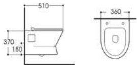
LX-1159 Rimless Siphonic One-piece Toilet Size:510x360x370mm Vitreous china S-trap,180mm Rounghing-in
