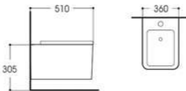
LX-1067 Bidet Size:510x360x305mm Vitreous china Fixing to wall with back
