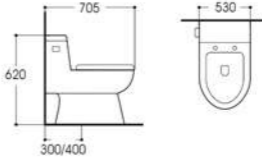
LX-2027 Siphonic One-piece Toilet Size:705x530x620mm Vitreous china S-trap,300/400mm Rounghing-in
