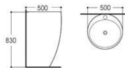
LX-8001 Pedestal Basin Size:500x500x830mm Vitreous china Fixing to wall with back
