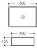
LX-5310 Art basin Size:600x400x120mm Vitreous china Above counter mounting
