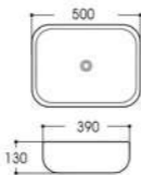
LX-7038 Art basin Size:500x390x130mm Vitreous china Above counter mounting
