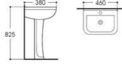
LX-5620F Pedestal Basin Size:460x380x825mm Vitreous china Fixing to wall with back
