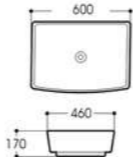
LX-9111 Art basin Size:600x460x170mm Vitreous china Above counter mounting
