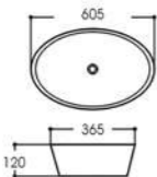
LX-5561 Art basin Size:605x365x120mm Vitreous china Above counter mounting
