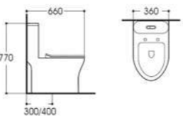
LX-2036 Siphonic One-piece Toilet Size:660x360x770mm Vitreous china S-trap,300/400mm Rounghing-in
