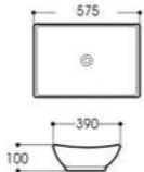
LX-5373 Art basin Size:575x390x100mm Vitreous china Above counter mounting
