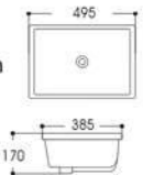
LX-6221 Under Counter Basin Outside Size:495x385x170mm 19 1/2"x15 1/4"x6" 3/4" Inside Size:435x325mm 17 1/8"x12 3/4" Under counter mounting
