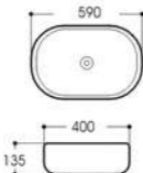
LX-5271 Art basin Size:590x400x135mm Vitreous china Above counter mounting
