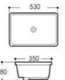
LX-6111 Under Counter Basin Outside Size:530x350x180mm 20 7/8"x13 3/4"x7 1/8" Inside Size:475x290mm 18 3/4"x11 3/8" Under counter mounting
