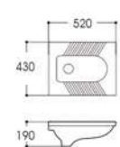
LX-3802 Squatting Pan W.C Size:520x430x190mm Vitreous china Fixing to wall with back
