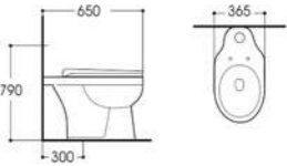
LX-1012 Wasdown Two-piece Toilet Size:650x365x790mm Vitreous china S-trap,300mm Rounghing-in
