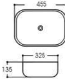
LX-7117 Art basin Size:455x325x135mm Vitreous china Above counter mounting
