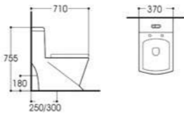
LX-2190 Rimless Siphonic One-piece Toilet Size:710x370x755mm Vitreous china S-trap,250/300mm Rounghing-in P-trap,180mm Rounghing-in
