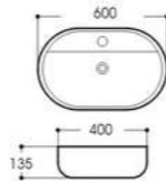
LX-5593 Art basin Size:600x400x135mm Vitreous china Above counter mounting
