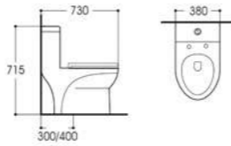
LX-2198 Rimless Siphonic One-piece Toilet Size:730x380x715mm Vitreous china S-trap,300/400 Rounghing-in
