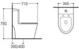
LX-2177 Rimless Siphonic One-piece Toilet Size:710x365x750mm Vitreous china S-trap,300/400 Rounghing-in
