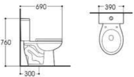
LX-2748A Siphonic Two-piece Toilet Size:690x390x760mm Vitreous china S-trap,300mm Rounghing-in
