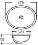
LX-6228 Under Counter Basin Outside Size:475x390x195mm 18 3/4"x15 3/8"x7 3/4" Inside Size:420x340mm 16 1/2"x13 3/8" Under counter mounting
