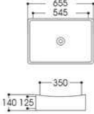
LX-5187A/5187B Art basin Size A:655x350x140mm Size B:545x350x125mm Above counter mounting
