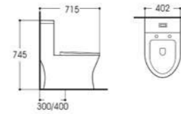
LX-2193 Rimless Siphonic One-piece Toilet Size:715x402x745mm Vitreous china S-trap,300/400 Rounghing-in
