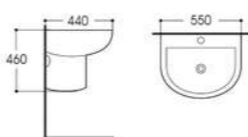
LX-3206H Wall-hung Basin Size:550x440x460mm Vitreous china Fixing to wall with back
