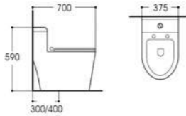
LX-2710 Siphonic One-piece Toilet Size:700x375x590mm Vitreous china S-trap,300/400mm Rounghing-in
