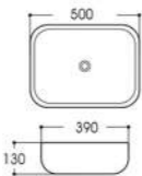
LX-7037 Art basin Size:500x390x130mm Vitreous china Above counter mounting
